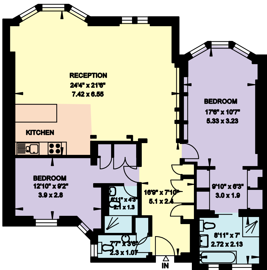
THIRD FLOOR
